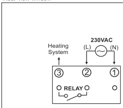
Figure 4 Electrical connections
